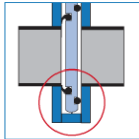
Type IC-SL. Gate valve for slurry, sludge and water removal.
